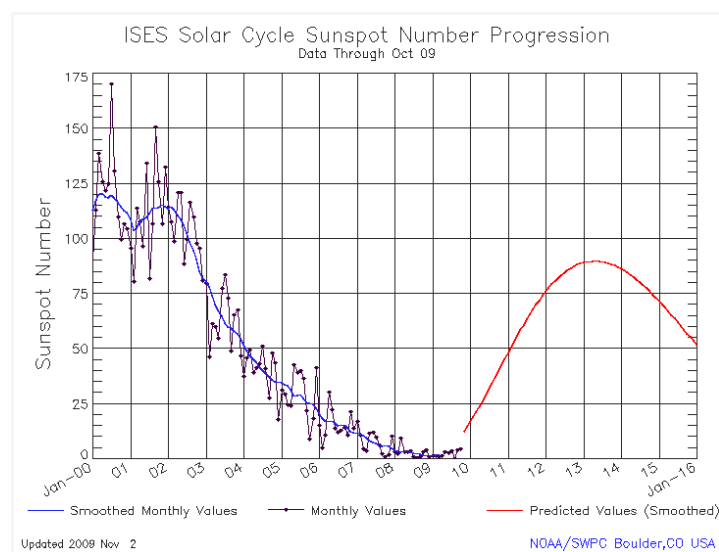
Fig 2: Solar cycle sunspot maximum will occur in the end of year 2013 according to the predictions made by NOAA Space Weather Prediction Center ( http://www.swpc.noaa.gov/SWN/index.html ). The solar cycle is usually estimated to about 11 years.
