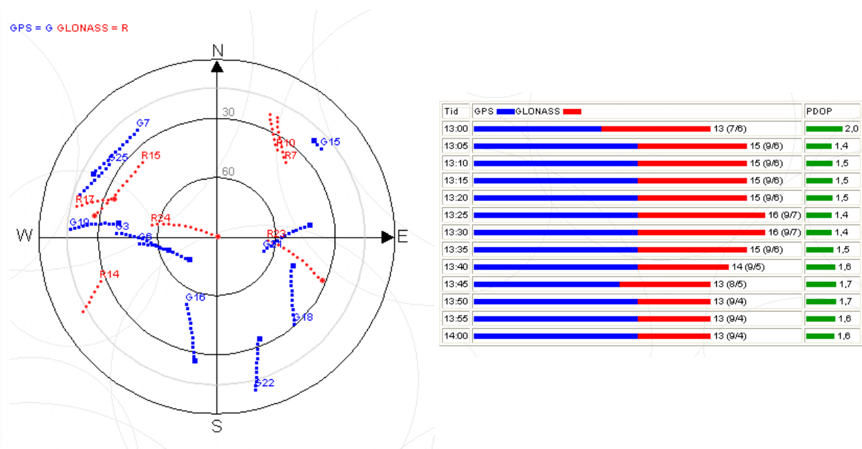
Fig 1: An example of a skyplot with an elevation cut off angle of 15 degrees and a table of the number of satellites available and the estimated PDOP for a specific time epoch (from http://www.swepos.com ).
