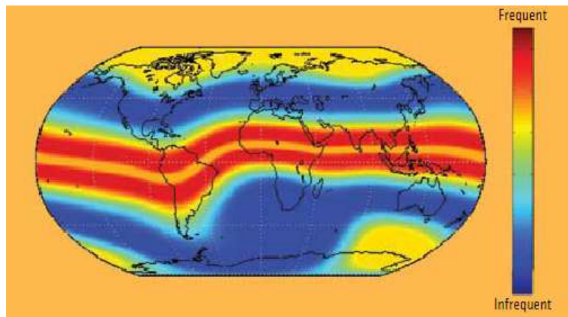
Fig 3: Ionospheric scintillation map which shows the effects of a solar maximum in different parts of the world, where the equator will be affected up to 100 days per year (KINTNER et al. 2009).
